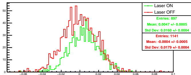
Run 4388 quartetwise, asym0: Beam ON
