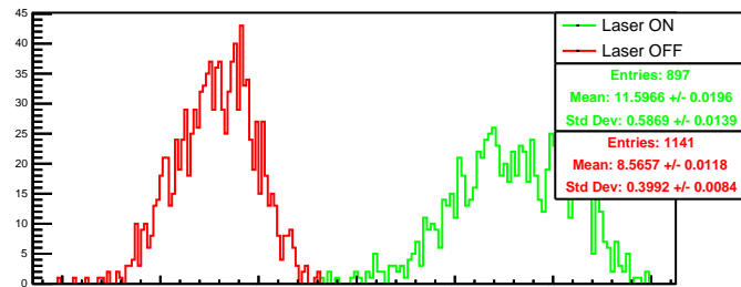
Run 4388 quartetwise, negH0: Beam ON
