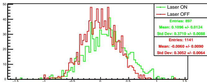
Run 4388 quartetwise, diff0: Beam ON
