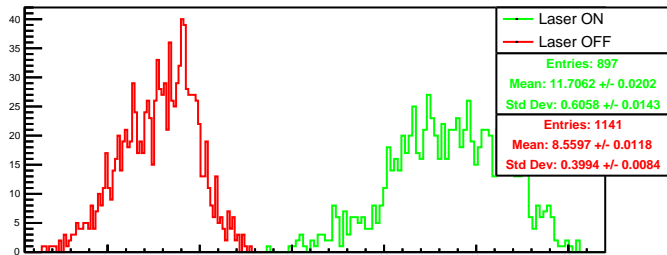
Run 4388 quartetwise, posH0: Beam ON
