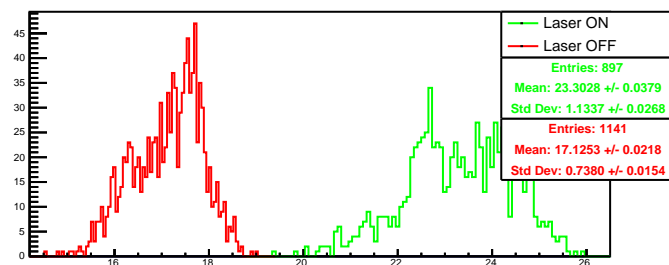
Run 4388 quartetwise, summ0: Beam ON
