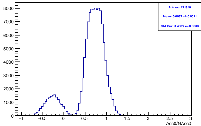
Run 4389 mpwise, acc0: Beam ON, Laser OFF
