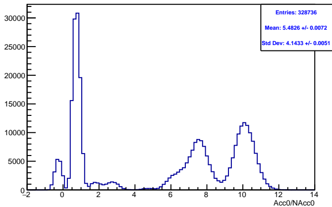
Run 4389 mpwise, acc0: Beam ON, Laser ON
