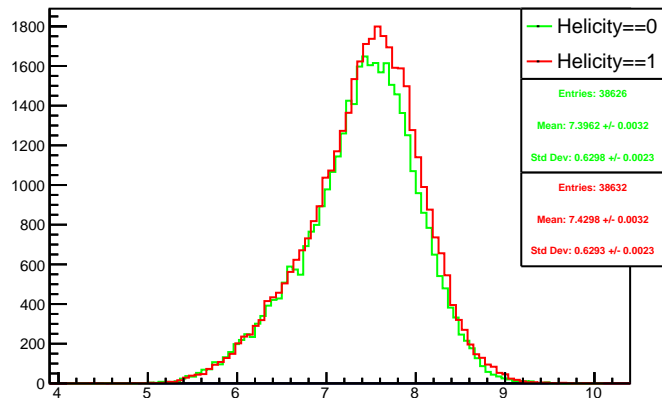
Run 4389 mpwise, acc0: Beam ON, Laser OFF
