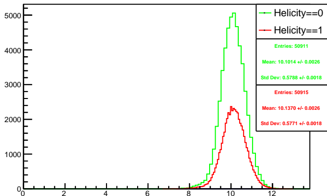
Run 4389 mpwise, acc0: Beam ON, Laser ON
