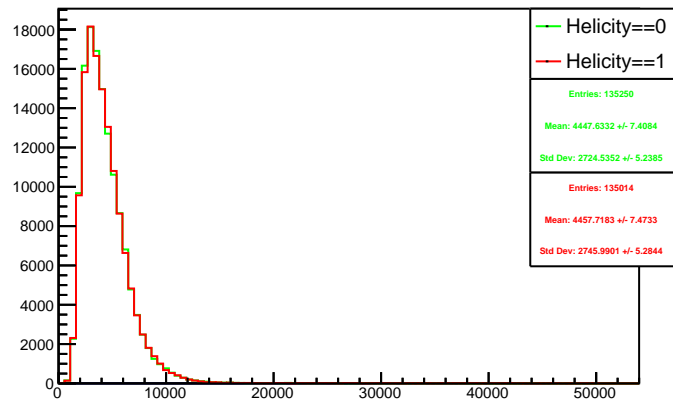
Run 4389 triggerwise, sums: Beam ON, Laser OFF
