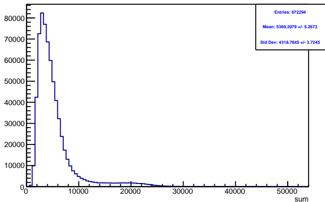
Run 4389 triggerwise, sums: All
