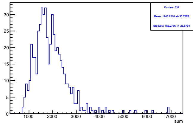
Run 4389 triggerwise, sums: Beam OFF
