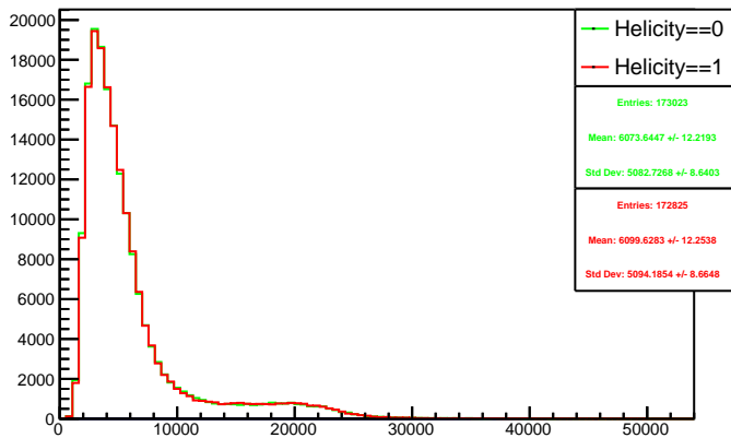
Run 4389 triggerwise, sums: Beam ON, Laser ON
