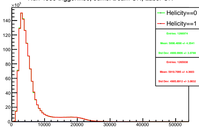
Run 4390 triggerwise, sums: Beam ON, Laser ON
