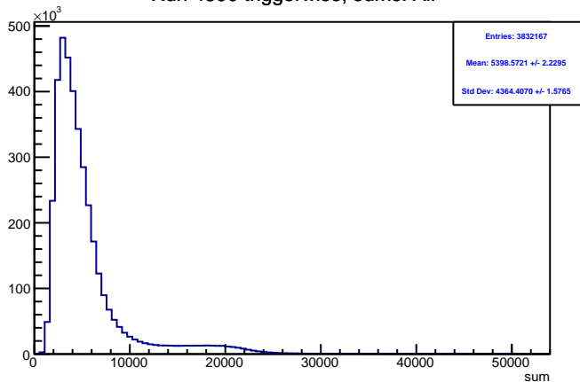
Run 4390 triggerwise, sums: All
