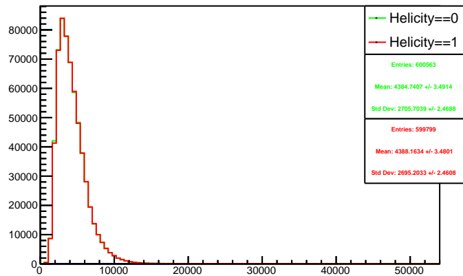
Run 4390 triggerwise, sums: Beam ON, Laser OFF
