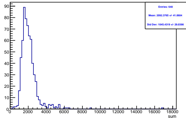
Run 4390 triggerwise, sums: Beam ON, Laser OFF
