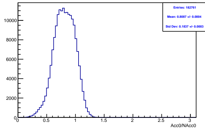
Run 4391 mpwise, acc0: Beam ON, Laser OFF
