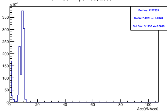
Run 4391 mpwise, acc0: All
