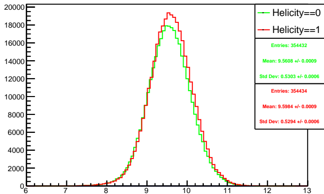
Run 4391 mpwise, acc0: Beam ON, Laser ON
