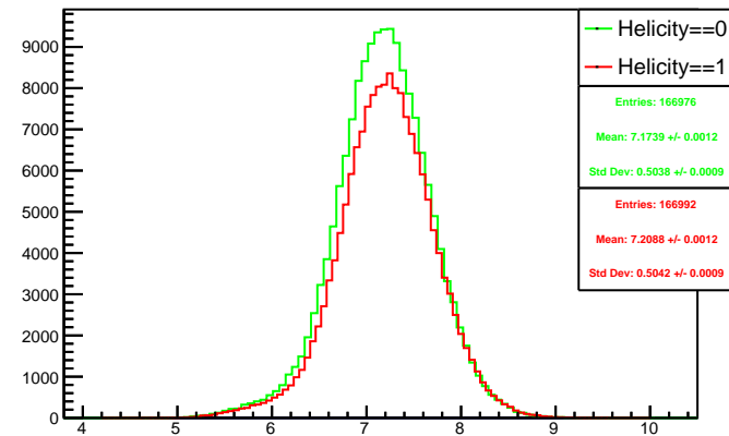
Run 4391 mpwise, acc0: Beam ON, Laser OFF
