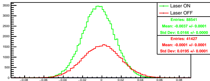
Run 4391 quartetwise, asym0: Beam ON
