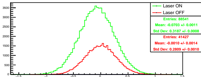
Run 4391 quartetwise, diff0: Beam ON
