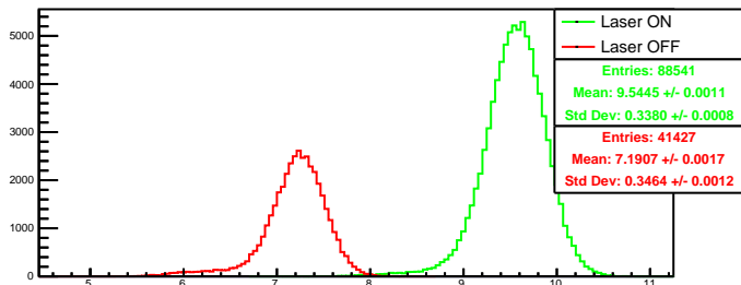
Run 4391 quartetwise, posH0: Beam ON
