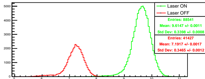
Run 4391 quartetwise, negH0: Beam ON
