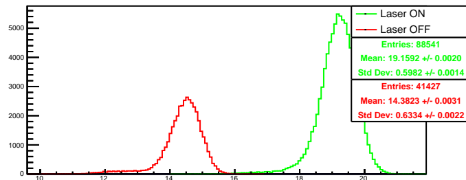
Run 4391 quartetwise, summ0: Beam ON
