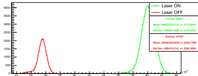
Run 4391 quartetwise, summ4: Beam ON
