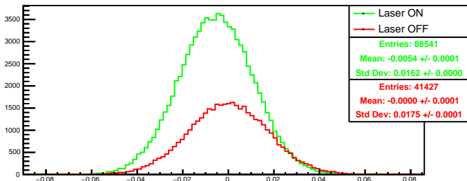
Run 4391 quartetwise, asym4: Beam ON
