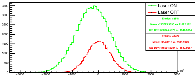
Run 4391 quartetwise, diff4: Beam ON
