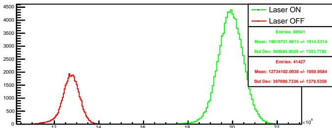
Run 4391 quartetwise, posH4: Beam ON
