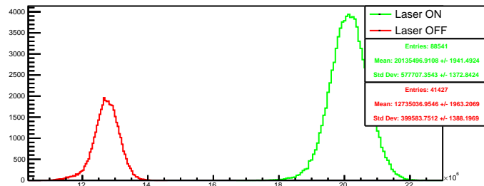
Run 4391 quartetwise, negH4: Beam ON
