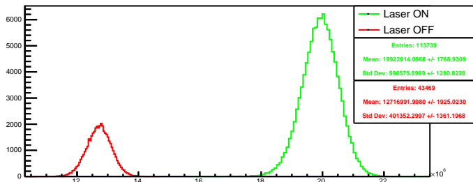
Run 4392 quartetwise, posH4: Beam ON
