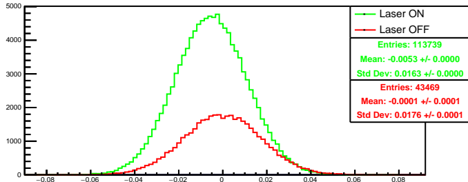
Run 4392 quartetwise, asym4: Beam ON
