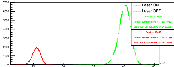
Run 4392 quartetwise, summ4: Beam ON
