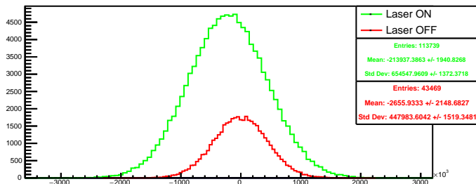
Run 4392 quartetwise, diff4: Beam ON
