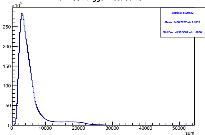
Run 4392 triggerwise, sums: All
