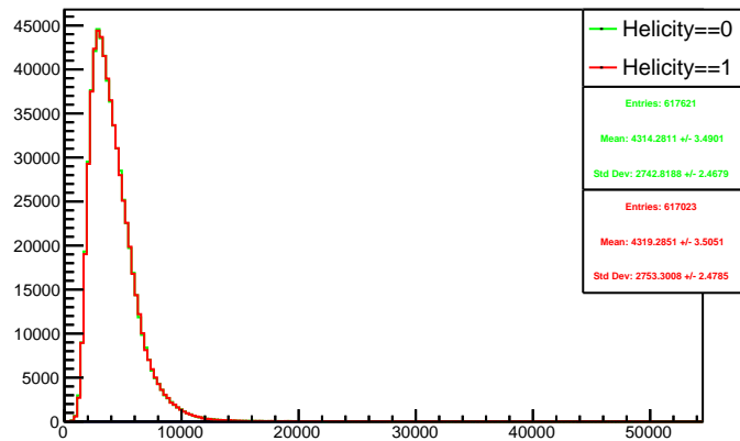
Run 4392 triggerwise, sums: Beam ON, Laser OFF
