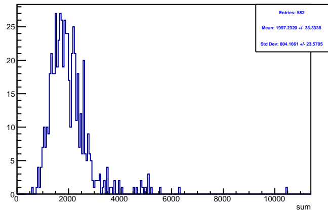
Run 4392 triggerwise, sums: Beam ON, Laser OFF
