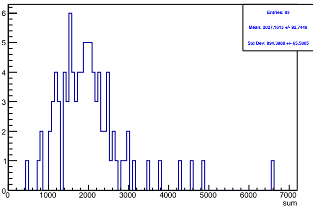
Run 4395 triggerwise, sums: Beam ON, Laser OFF
