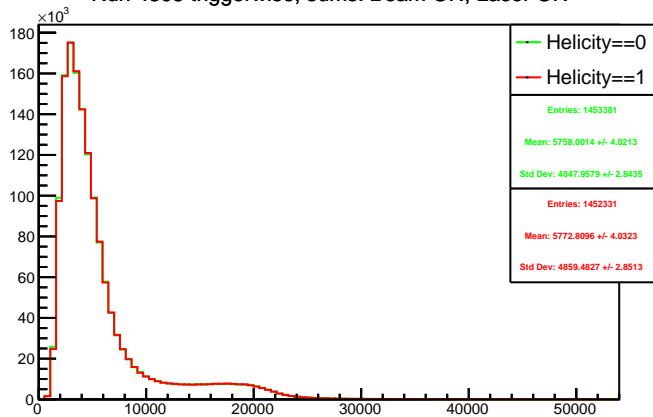
Run 4395 triggerwise, sums: Beam ON, Laser ON
