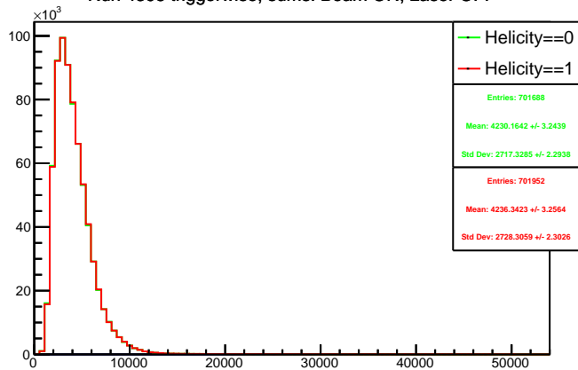
Run 4395 triggerwise, sums: Beam ON, Laser OFF
