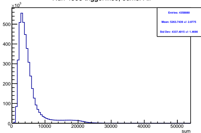
Run 4395 triggerwise, sums: All
