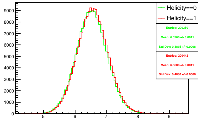
Run 4396 mpwise, acc0: Beam ON, Laser OFF
