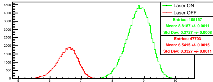
Run 4396 quartetwise, negH0: Beam ON
