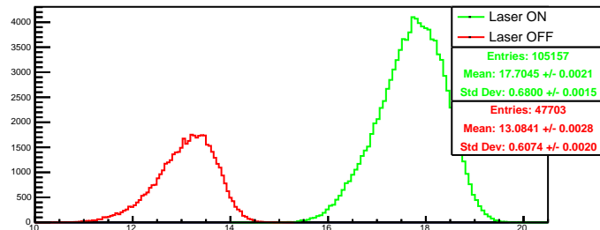
Run 4396 quartetwise, summ0: Beam ON
