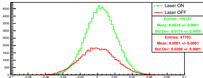
Run 4396 quartetwise, asym0: Beam ON
