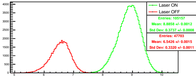
Run 4396 quartetwise, posH0: Beam ON
