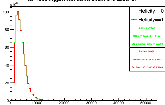
Run 4396 triggerwise, sums: Beam ON, Laser OFF
