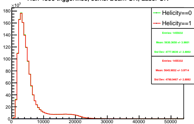
Run 4396 triggerwise, sums: Beam ON, Laser ON
