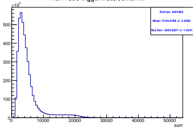
Run 4396 triggerwise, sums: All
