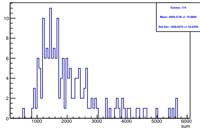
Run 4397 triggerwise, sums: Beam ON, Laser OFF
