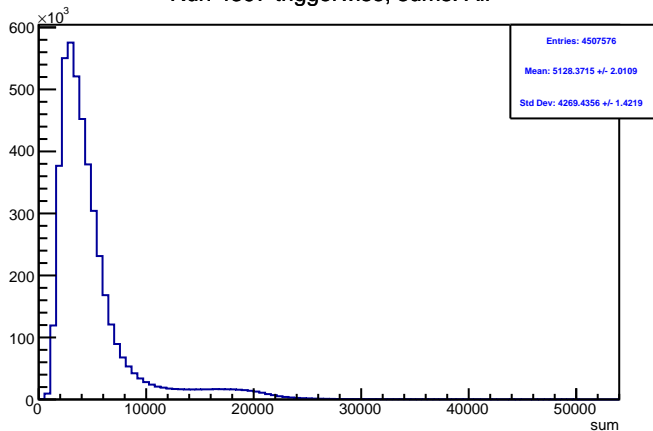
Run 4397 triggerwise, sums: All
