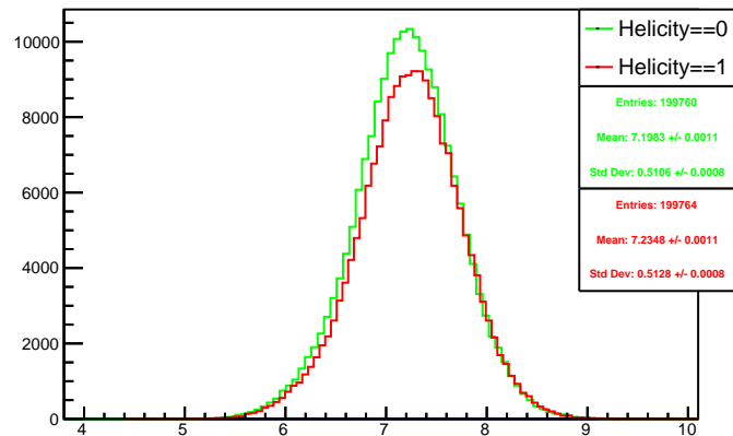
Run 4400 mpwise, acc0: Beam ON, Laser OFF
