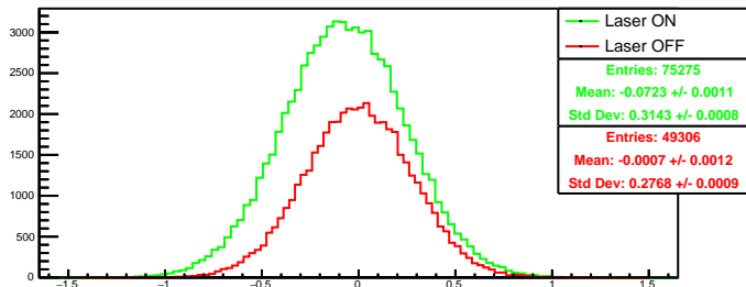
Run 4400 quartetwise, diff0: Beam ON
