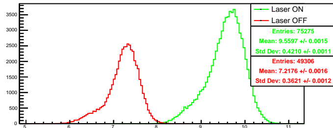
Run 4400 quartetwise, negH0: Beam ON
