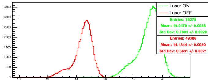
Run 4400 quartetwise, summ0: Beam ON
