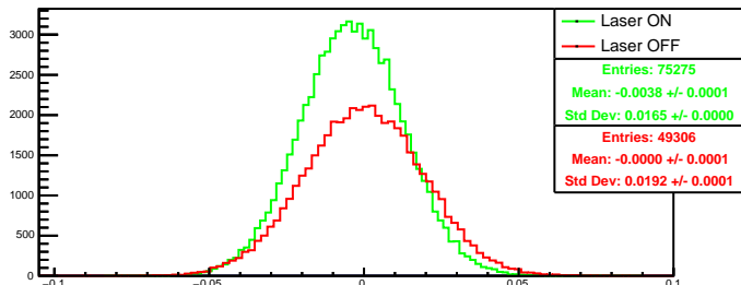
Run 4400 quartetwise, asym0: Beam ON
