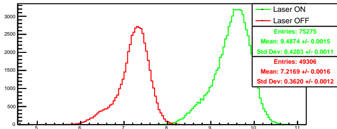
Run 4400 quartetwise, posH0: Beam ON
