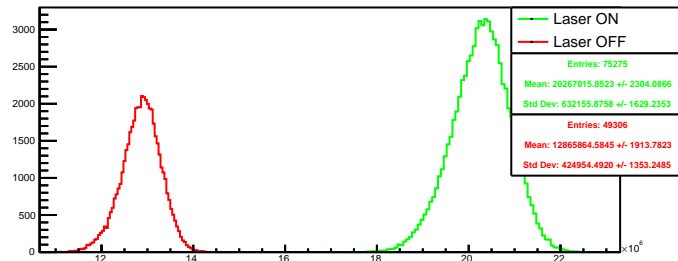
Run 4400 quartetwise, negH4: Beam ON
