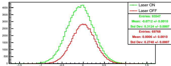
Run 4401 quartetwise, diff0: Beam ON
