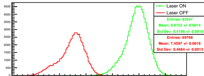
Run 4401 quartetwise, negH0: Beam ON
