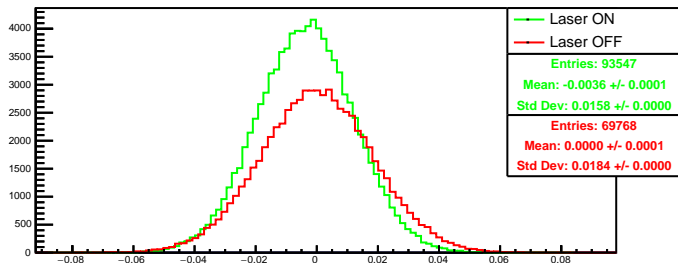
Run 4401 quartetwise, asym0: Beam ON
