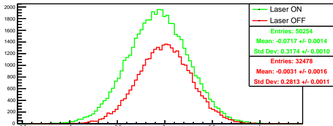
Run 4403 quartetwise, diff0: Beam ON
