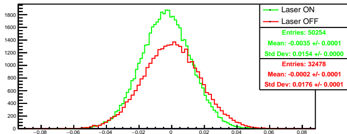
Run 4403 quartetwise, asym0: Beam ON
