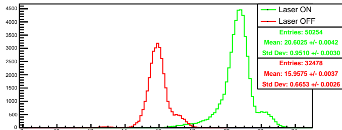
Run 4403 quartetwise, summ0: Beam ON
