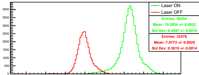
Run 4403 quartetwise, posH0: Beam ON
