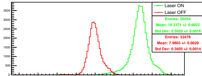
Run 4403 quartetwise, negH0: Beam ON
