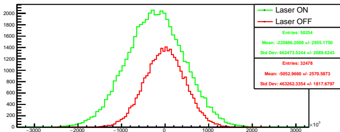
Run 4403 quartetwise, diff4: Beam ON
