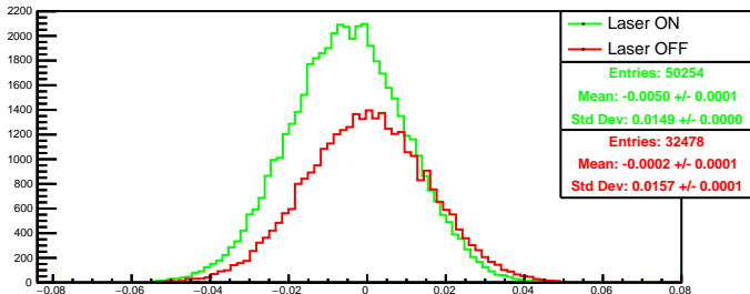
Run 4403 quartetwise, asym4: Beam ON
