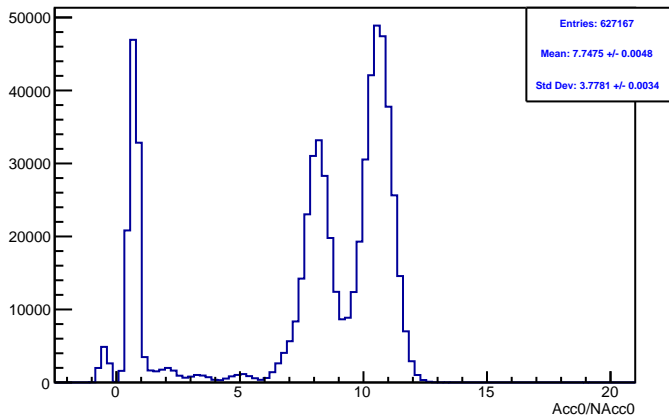
Run 4404 mpwise, acc0: Beam ON, Laser ON
