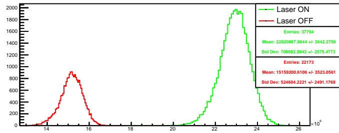
Run 4404 quartetwise, negH4: Beam ON
