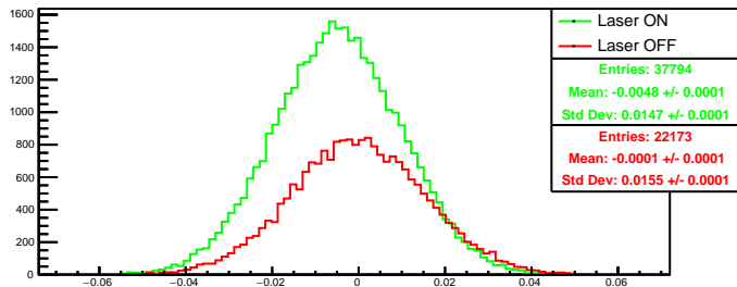
Run 4404 quartetwise, asym4: Beam ON
