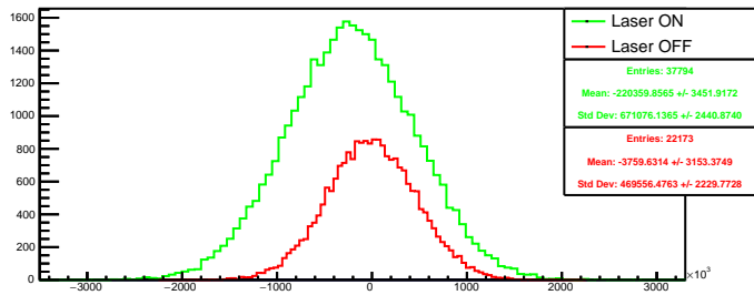
Run 4404 quartetwise, diff4: Beam ON
