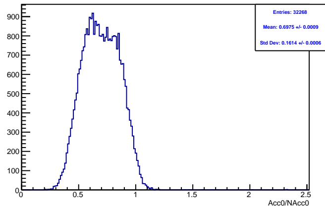
Run 4412 mpwise, acc0: Beam ON, Laser OFF
