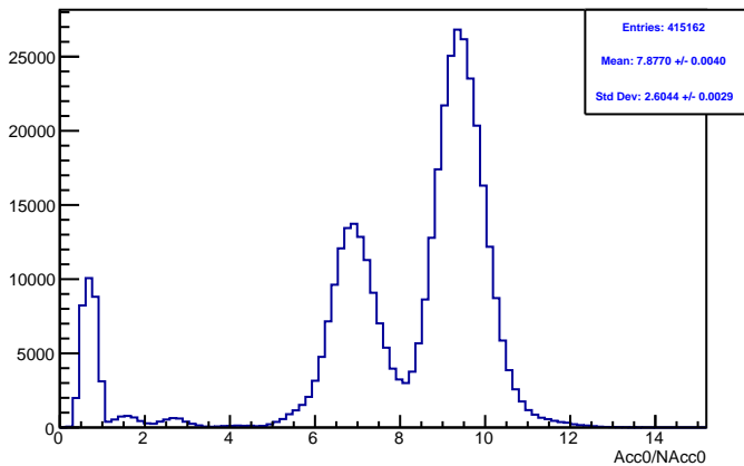
Run 4412 mpwise, acc0: Beam ON, Laser ON
