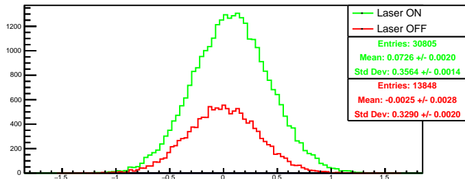
Run 4412 quartetwise, diff0: Beam ON
