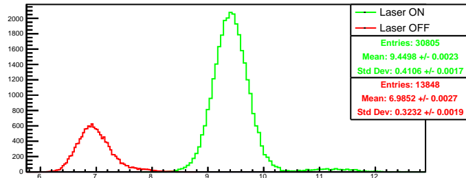
Run 4412 quartetwise, negH0: Beam ON
