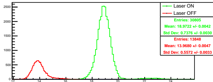
Run 4412 quartetwise, summ0: Beam ON
