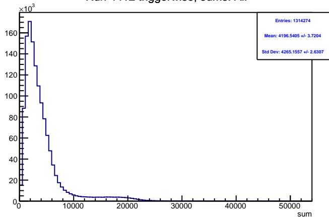
Run 4412 triggerwise, sums: All
