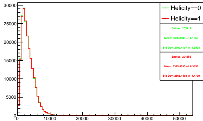
Run 4412 triggerwise, sums: Beam ON, Laser OFF
