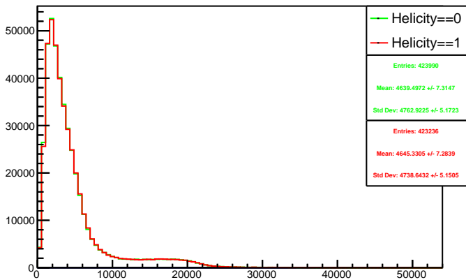
Run 4412 triggerwise, sums: Beam ON, Laser ON
