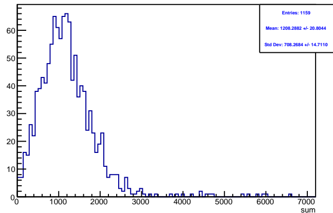
Run 4412 triggerwise, sums: Beam OFF
