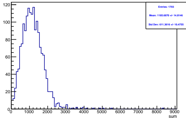
Run 4413 triggerwise, sums: Beam ON, Laser OFF
