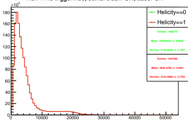
Run 4413 triggerwise, sums: Beam ON, Laser ON
