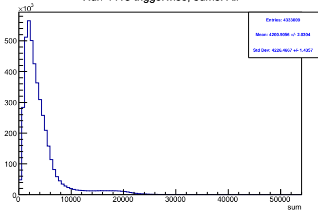
Run 4413 triggerwise, sums: All
