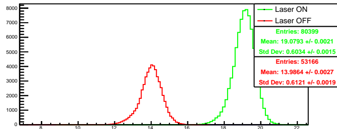
Run 4415 quartetwise, summ0: Beam ON
