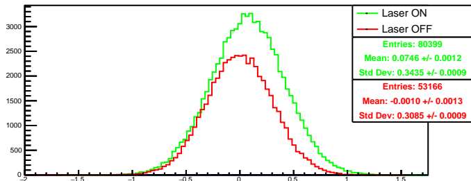
Run 4415 quartetwise, diff0: Beam ON
