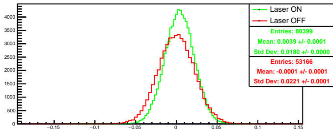
Run 4415 quartetwise, asym0: Beam ON
