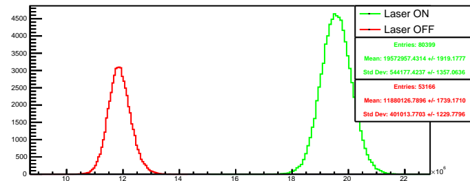
Run 4415 quartetwise, negH4: Beam ON
