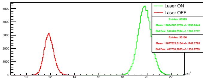
Run 4415 quartetwise, posH4: Beam ON
