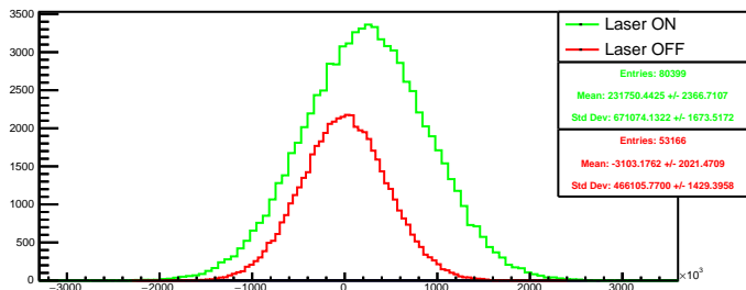
Run 4415 quartetwise, diff4: Beam ON
