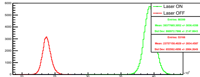
Run 4415 quartetwise, summ4: Beam ON
