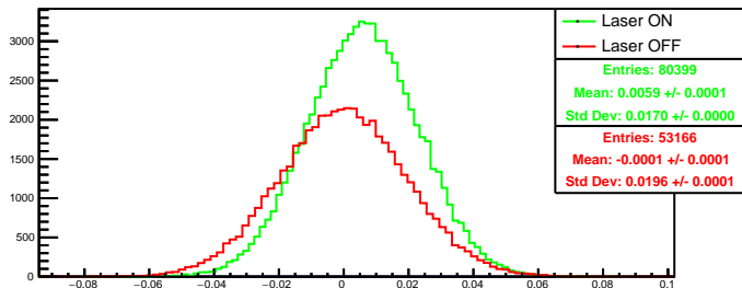
Run 4415 quartetwise, asym4: Beam ON
