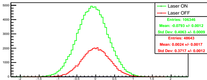
Run 4430 quartetwise, diff0: Beam ON
