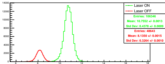
Run 4430 quartetwise, posH0: Beam ON
