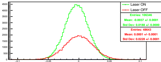
Run 4430 quartetwise, asym0: Beam ON
