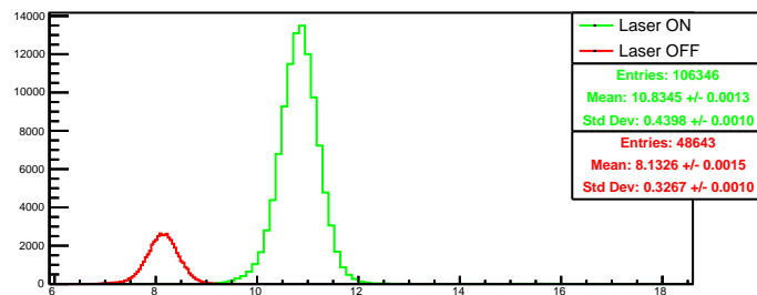
Run 4430 quartetwise, negH0: Beam ON
