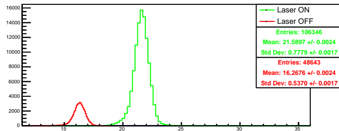
Run 4430 quartetwise, summ0: Beam ON
