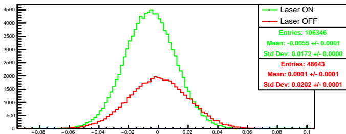
Run 4430 quartetwise, asym4: Beam ON
