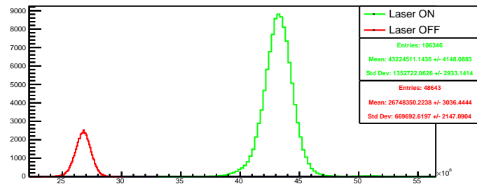
Run 4430 quartetwise, summ4: Beam ON
