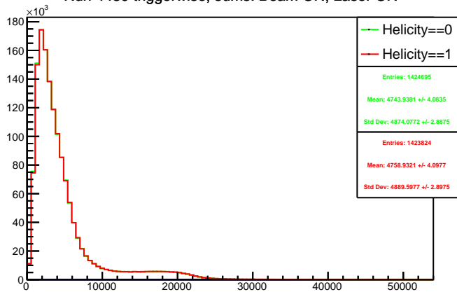
Run 4430 triggerwise, sums: Beam ON, Laser ON
