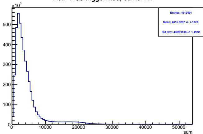
Run 4430 triggerwise, sums: All
