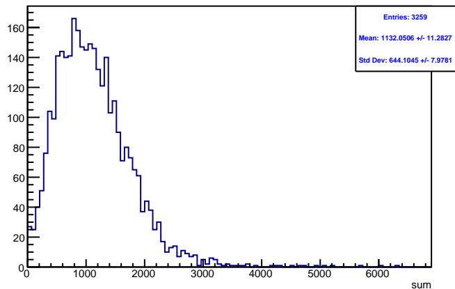
Run 4430 triggerwise, sums: Beam ON, Laser OFF
