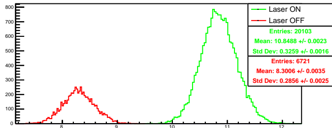
Run 4433 quartetwise, posH0: Beam ON
