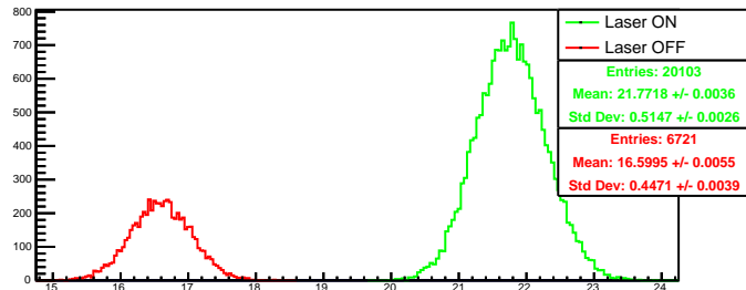
Run 4433 quartetwise, summ0: Beam ON
