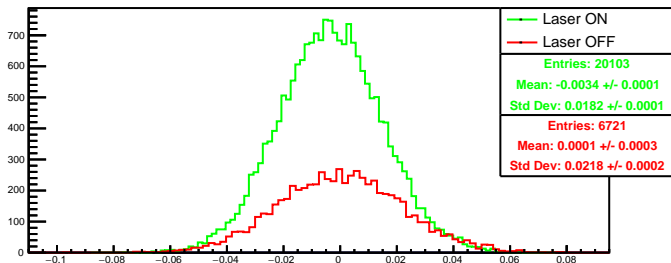
Run 4433 quartetwise, asym0: Beam ON
