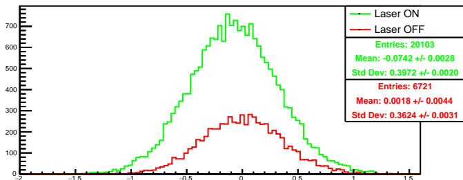
Run 4433 quartetwise, diff0: Beam ON
