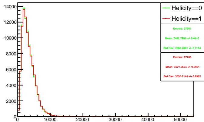
Run 4433 triggerwise, sums: Beam ON, Laser OFF
