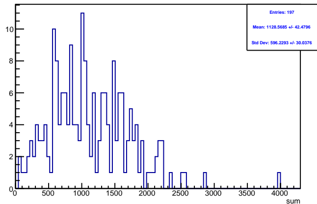
Run 4433 triggerwise, sums: Beam OFF
