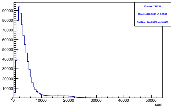
Run 4433 triggerwise, sums: All
