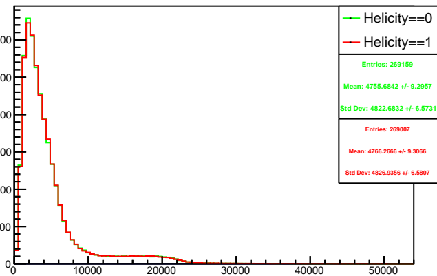
Run 4433 triggerwise, sums: Beam ON, Laser ON
