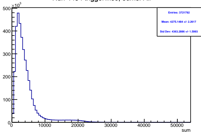
Run 4434 triggerwise, sums: All
