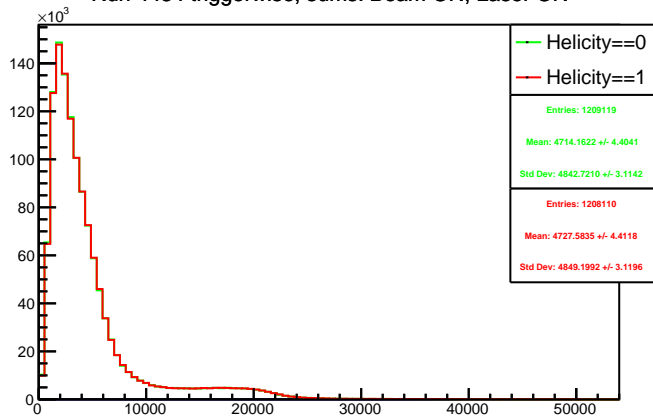
Run 4434 triggerwise, sums: Beam ON, Laser ON
