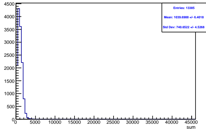
Run 4434 triggerwise, sums: Beam OFF
