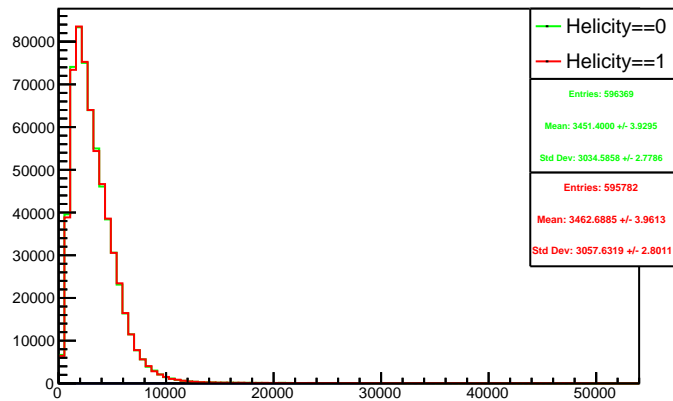
Run 4434 triggerwise, sums: Beam ON, Laser OFF
