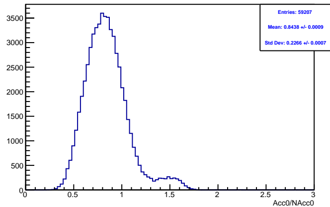
Run 4435 mpwise, acc0: Beam ON, Laser OFF
