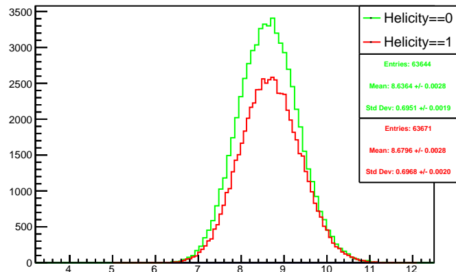
Run 4435 mpwise, acc0: Beam ON, Laser OFF
