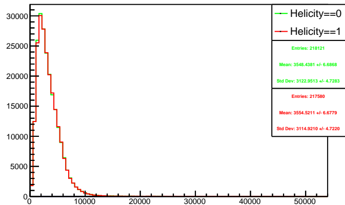
Run 4435 triggerwise, sums: Beam ON, Laser OFF
