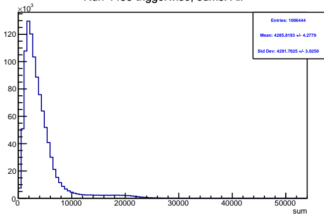
Run 4435 triggerwise, sums: All
