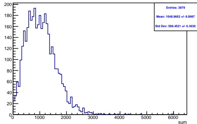
Run 4435 triggerwise, sums: Beam OFF
