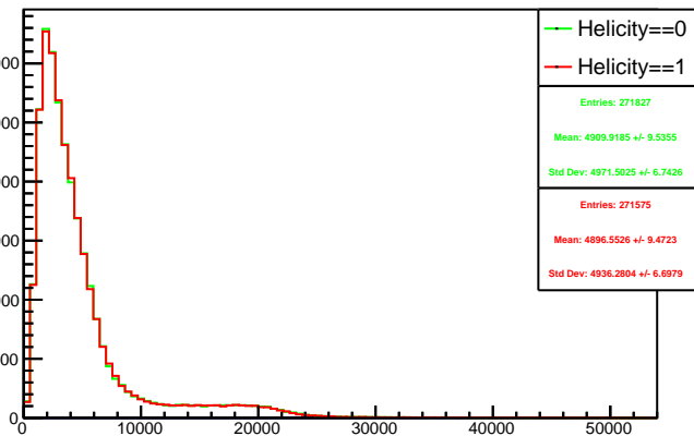
Run 4435 triggerwise, sums: Beam ON, Laser ON
