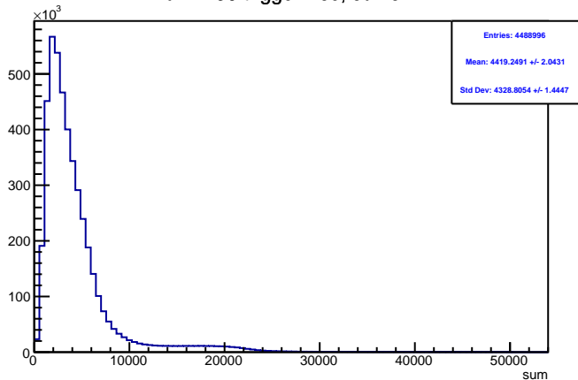
Run 4436 triggerwise, sums: All
