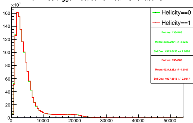
Run 4436 triggerwise, sums: Beam ON, Laser ON
