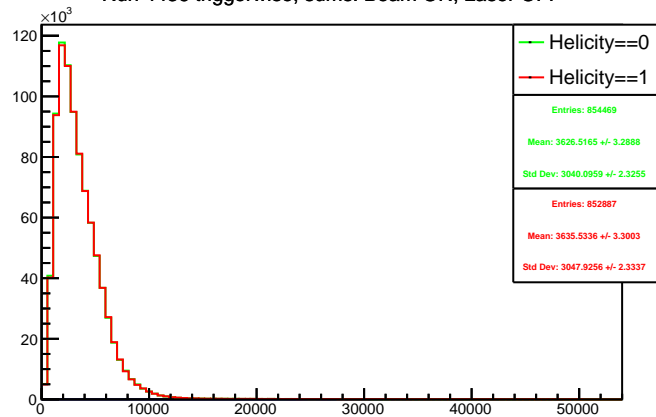
Run 4436 triggerwise, sums: Beam ON, Laser OFF
