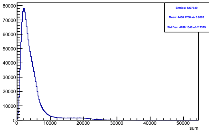
Run 4437 triggerwise, sums: Beam ON, Laser ON
