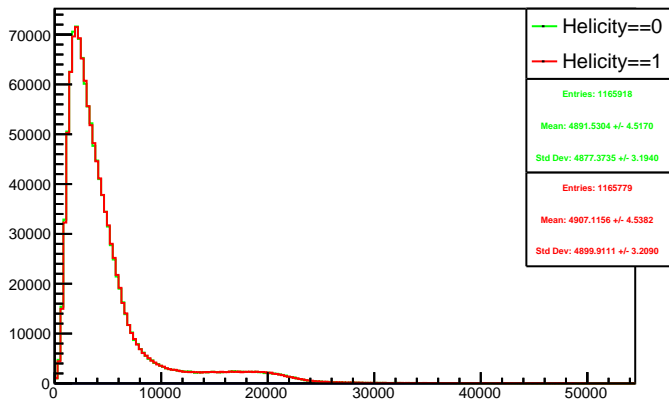
Run 4438 triggerwise, sums: Beam ON, Laser ON
