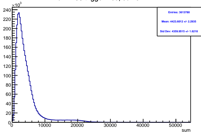
Run 4438 triggerwise, sums: All
