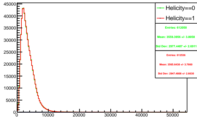
Run 4438 triggerwise, sums: Beam ON, Laser OFF
