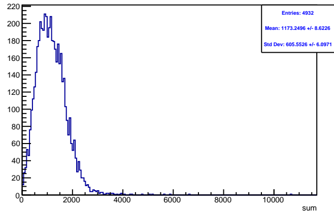
Run 4438 triggerwise, sums: Beam OFF
