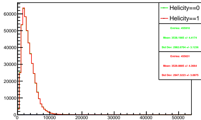
Run 4440 triggerwise, sums: Beam ON, Laser OFF
