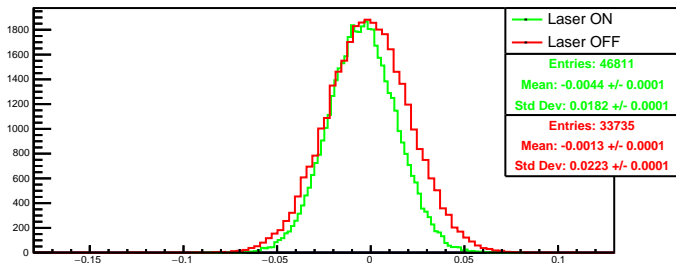
Run 4445 quartetwise, asym0: Beam ON
