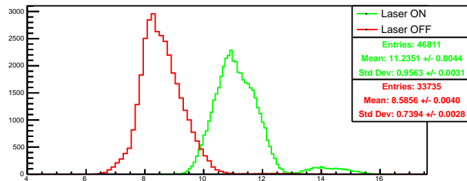
Run 4445 quartetwise, negH0: Beam ON
