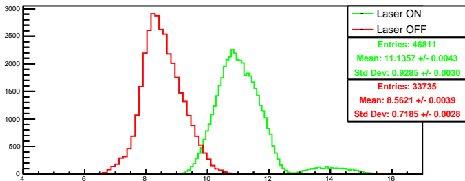
Run 4445 quartetwise, posH0: Beam ON
