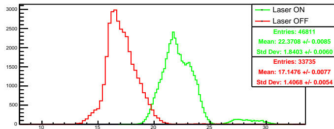
Run 4445 quartetwise, summ0: Beam ON
