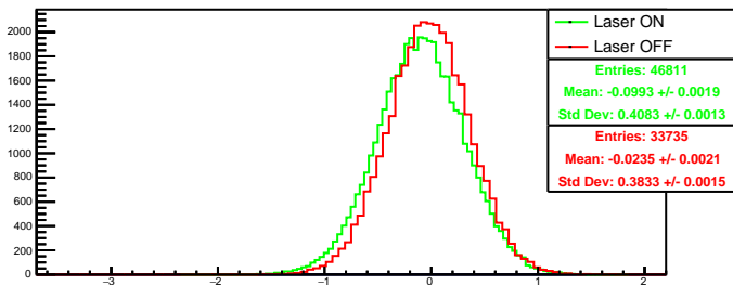
Run 4445 quartetwise, diff0: Beam ON
