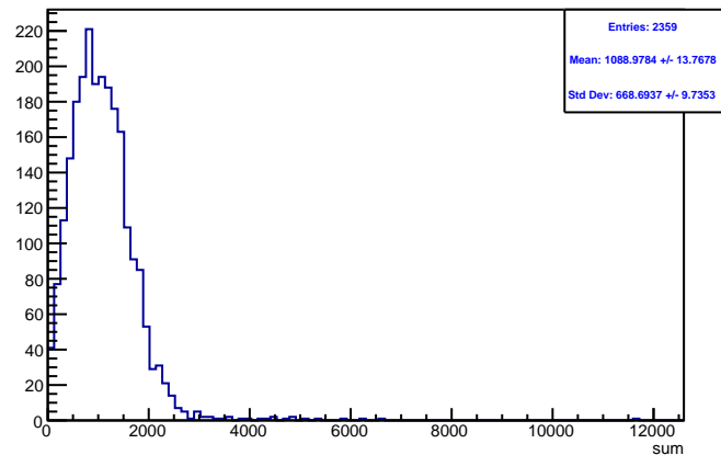
Run 4445 triggerwise, sums: Beam ON, Laser OFF
