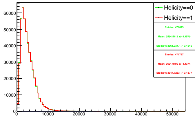
Run 4445 triggerwise, sums: Beam ON, Laser OFF
