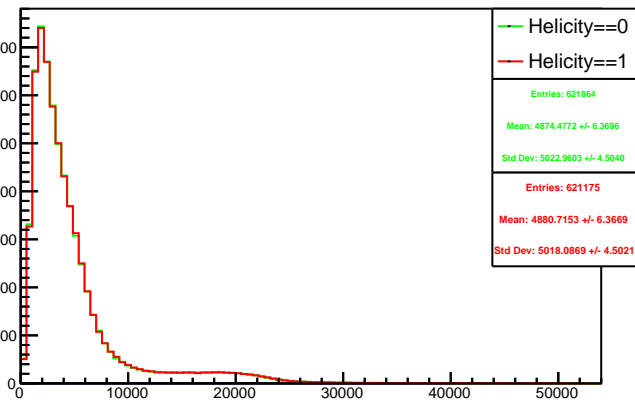
Run 4445 triggerwise, sums: Beam ON, Laser ON
