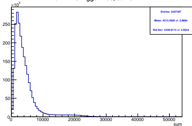
Run 4445 triggerwise, sums: All
