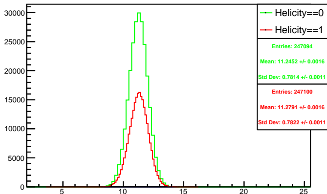
Run 4446 mpwise, acc0: Beam ON, Laser ON
