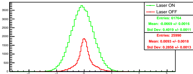
Run 4446 quartetwise, diff0: Beam ON
