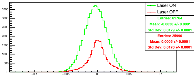
Run 4446 quartetwise, asym0: Beam ON
