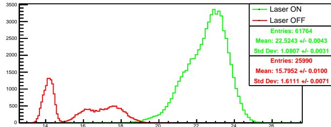
Run 4446 quartetwise, summ0: Beam ON
