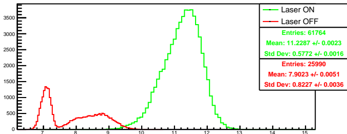
Run 4446 quartetwise, posH0: Beam ON
