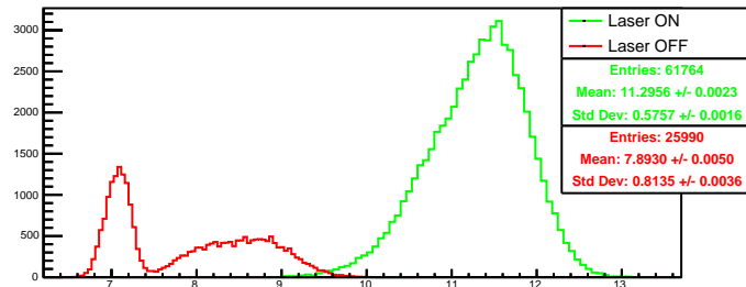
Run 4446 quartetwise, negH0: Beam ON
