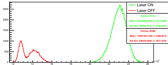
Run 4446 quartetwise, negH4: Beam ON
