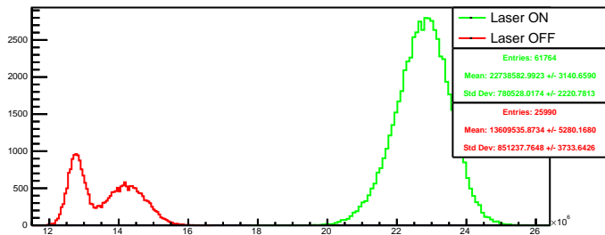
Run 4446 quartetwise, posH4: Beam ON
