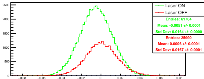
Run 4446 quartetwise, asym4: Beam ON
