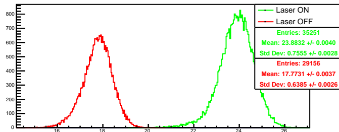
Run 4447 quartetwise, summ0: Beam ON
