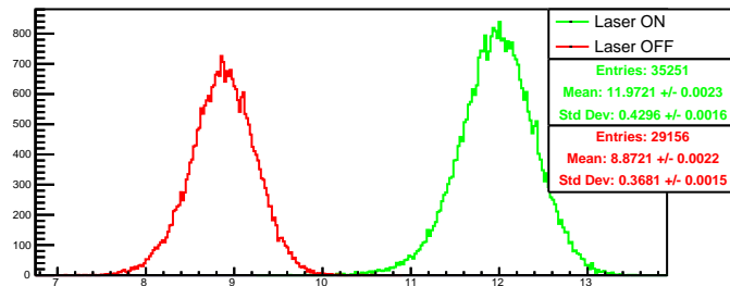
Run 4447 quartetwise, negH0: Beam ON
