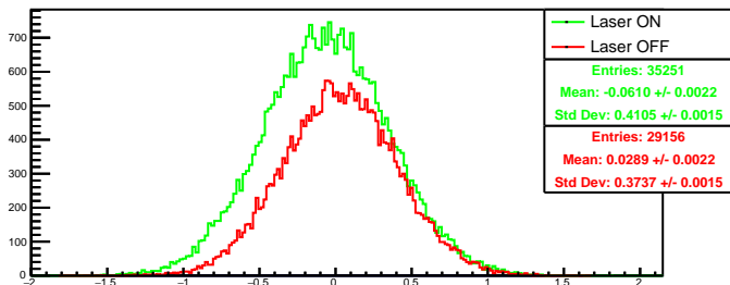
Run 4447 quartetwise, diff0: Beam ON
