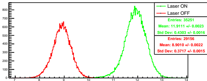
Run 4447 quartetwise, posH0: Beam ON
