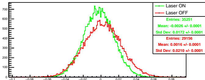
Run 4447 quartetwise, asym0: Beam ON
