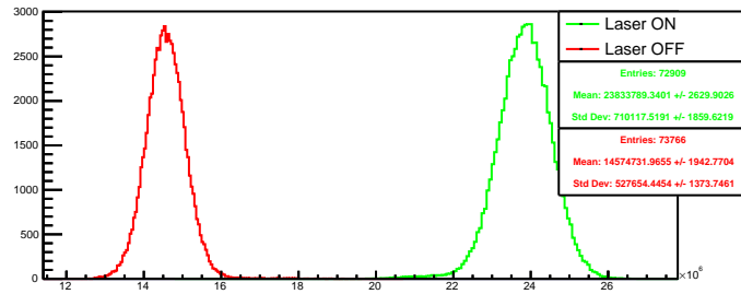
Run 4448 quartetwise, negH4: Beam ON
