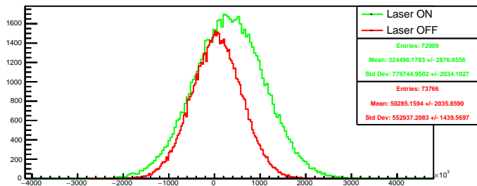
Run 4448 quartetwise, diff4: Beam ON
