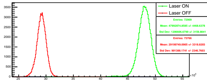
Run 4448 quartetwise, summ4: Beam ON
