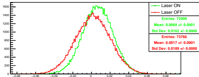
Run 4448 quartetwise, asym4: Beam ON
