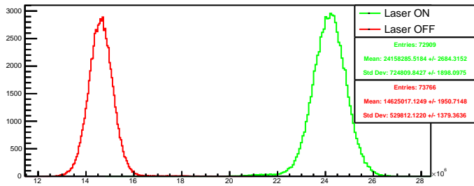
Run 4448 quartetwise, posH4: Beam ON
