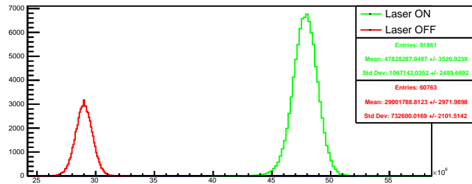
Run 4449 quartetwise, summ4: Beam ON
