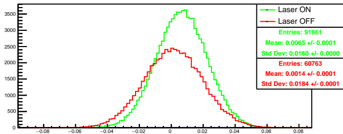
Run 4449 quartetwise, asym4: Beam ON
