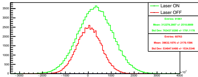
Run 4449 quartetwise, diff4: Beam ON
