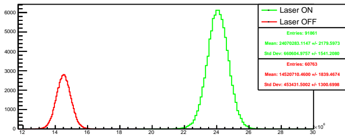
Run 4449 quartetwise, posH4: Beam ON
