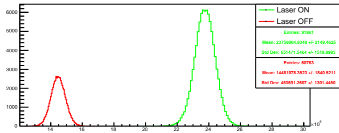
Run 4449 quartetwise, negH4: Beam ON
