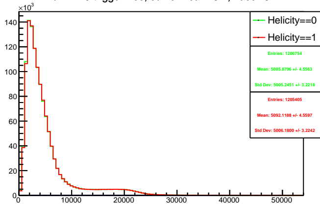
Run 4449 triggerwise, sums: Beam ON, Laser ON
