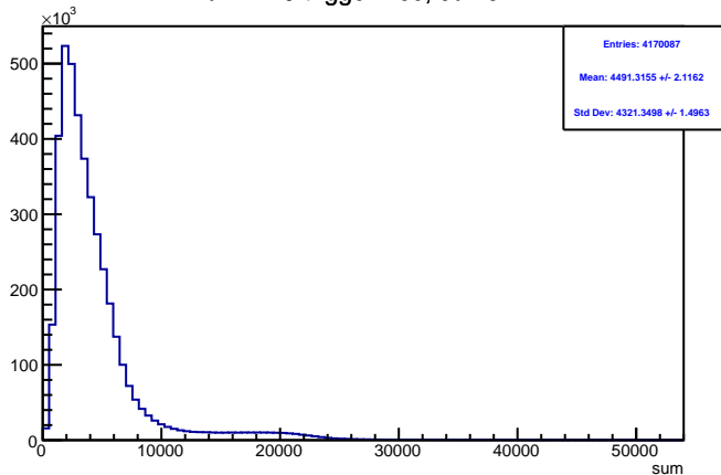
Run 4449 triggerwise, sums: All
