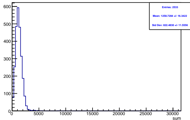
Run 4449 triggerwise, sums: Beam OFF
