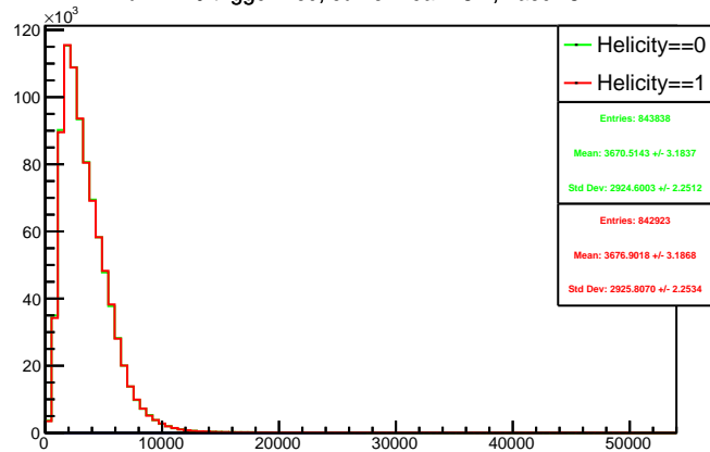
Run 4449 triggerwise, sums: Beam ON, Laser OFF
