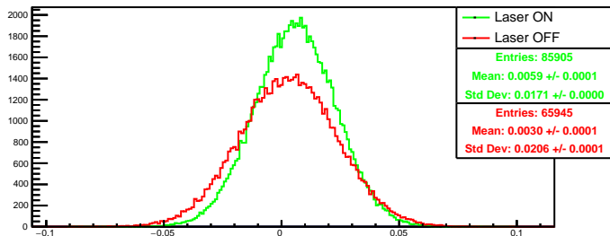
Run 4450 quartetwise, asym0: Beam ON
