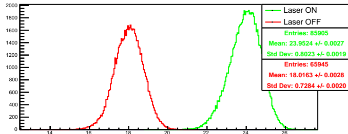
Run 4450 quartetwise, summ0: Beam ON
