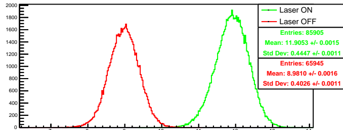
Run 4450 quartetwise, negH0: Beam ON
