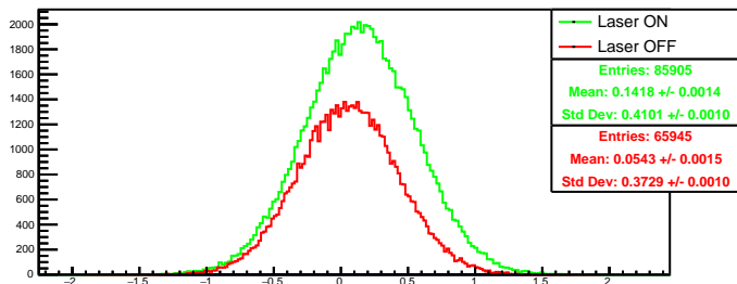
Run 4450 quartetwise, diff0: Beam ON
