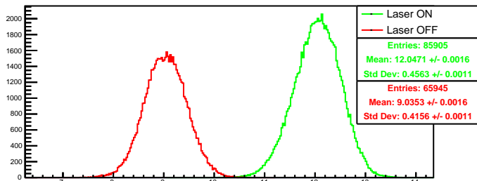
Run 4450 quartetwise, posH0: Beam ON
